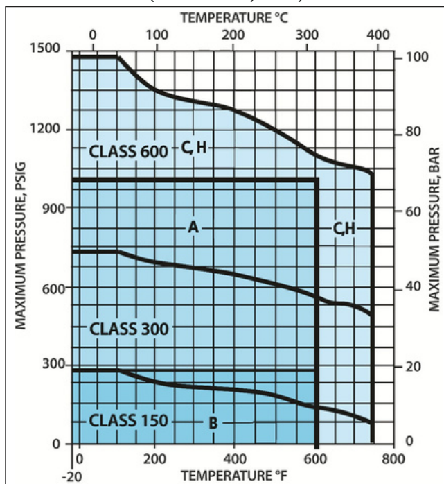
Figure 2. Trim Chart For Carbon Steel Body (ASTM A216, WCB)
