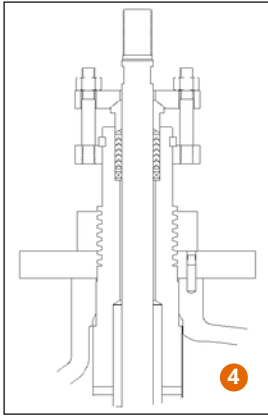
Figure 4. The bonnet for valves 1" through 8" (DN25 – 200) utilizes a simple unionnut construction in conjunction with a pressure seal to ensure zero leakage.
