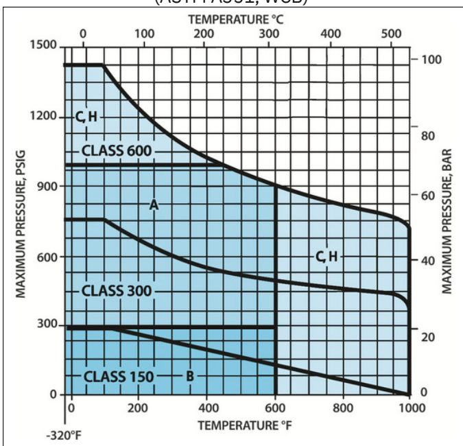
Figure 1. Trim Chart For Stainless Steel Body (ASTM A351, WCB)
