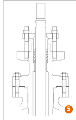
Figure 5. The bonnet for 10" through 16" (DN250 – 400) valves utilizes a flanged connection and flat metal gasket.
