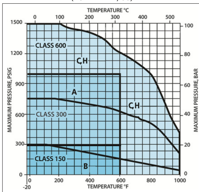
Figure 3. Trim Chart For Chrome-Moly Body (ASTM A217, C5)
